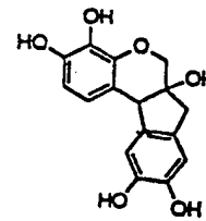
HEMATOXYLIN
